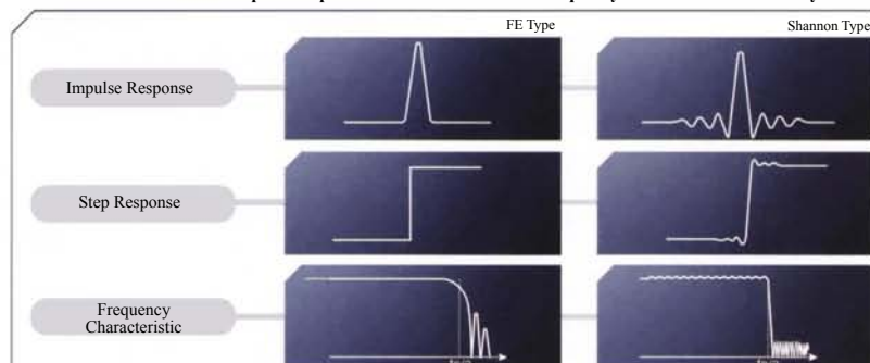
The differences between the impulse response characteristic and the frequency characteristic decided by DAC type
